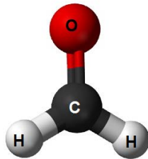
Formaldehyde Structure – CH 2 O
