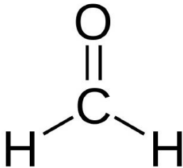
Formaldehyde Structure – CH 2 O
